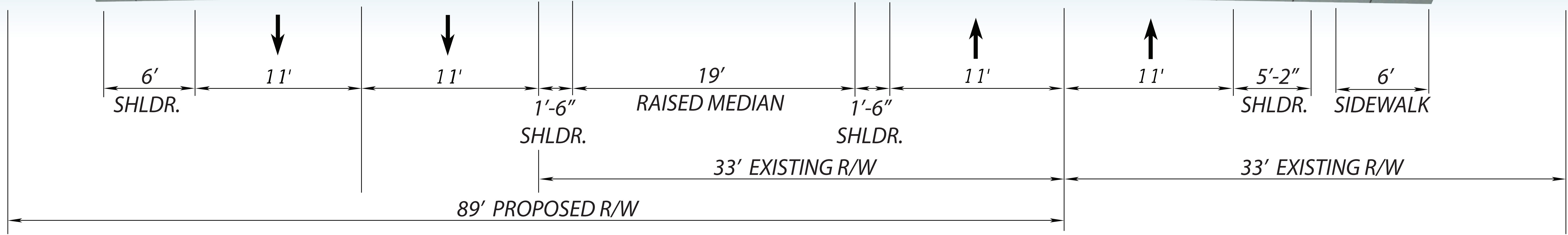
PROPOSED BRIDGE TYPICAL SECTION - ORANGE AVENUE OVER ST. MARKS TRAIL (BRIDGE 550171)
