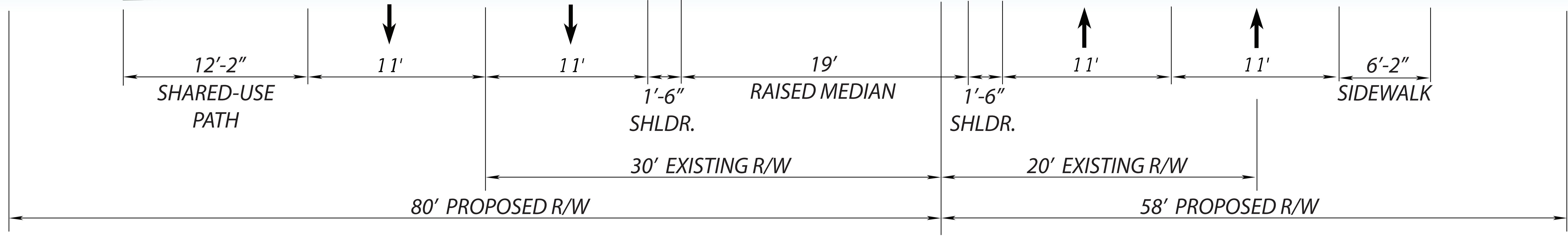
PROPOSED BRIDGE TYPICAL SECTION - ORANGE AVENUE OVER BLACK CREEK (BRIDGE 550037)
