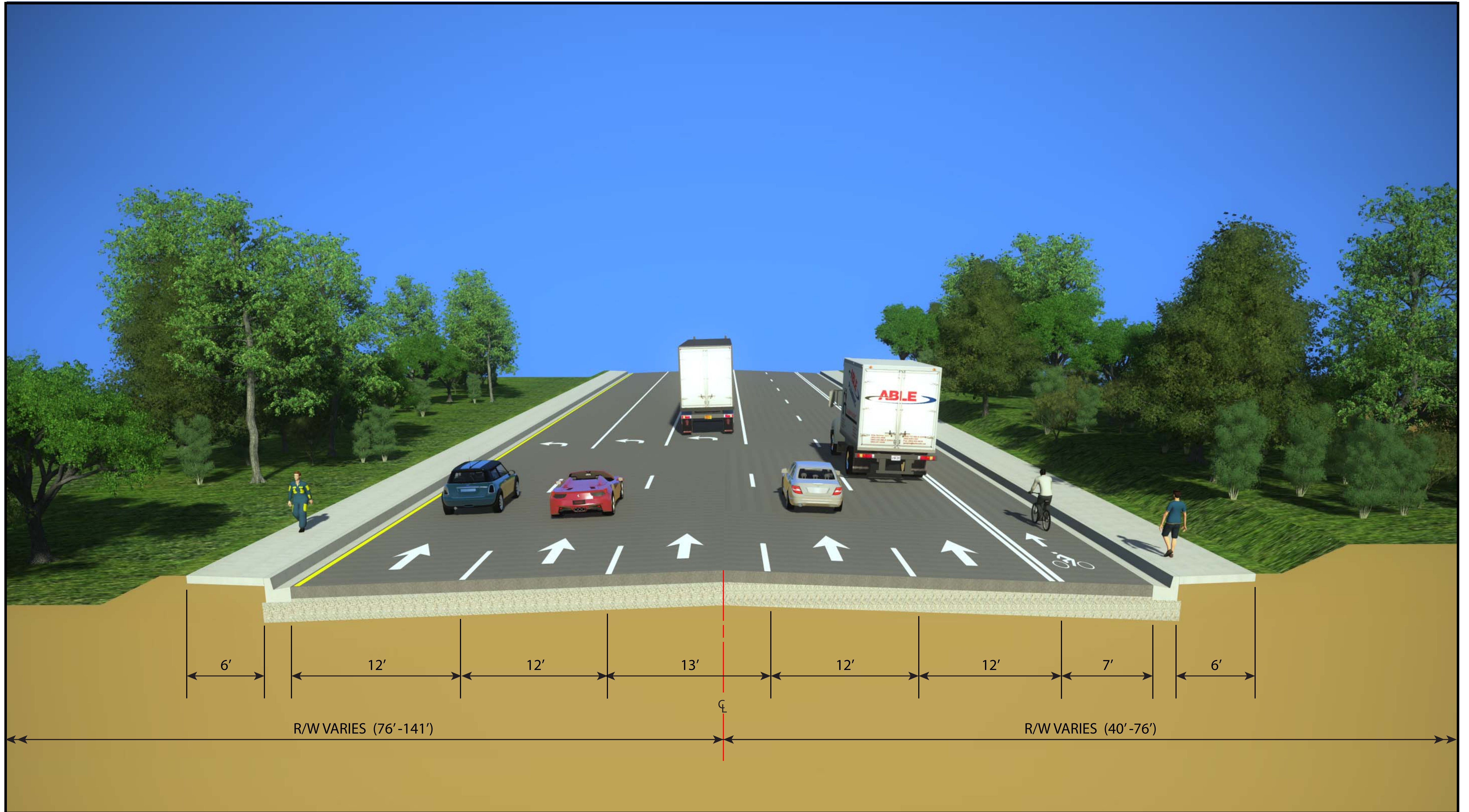
Typical Section - Segment 5 - S.R. 363 (Woodville Highway)
