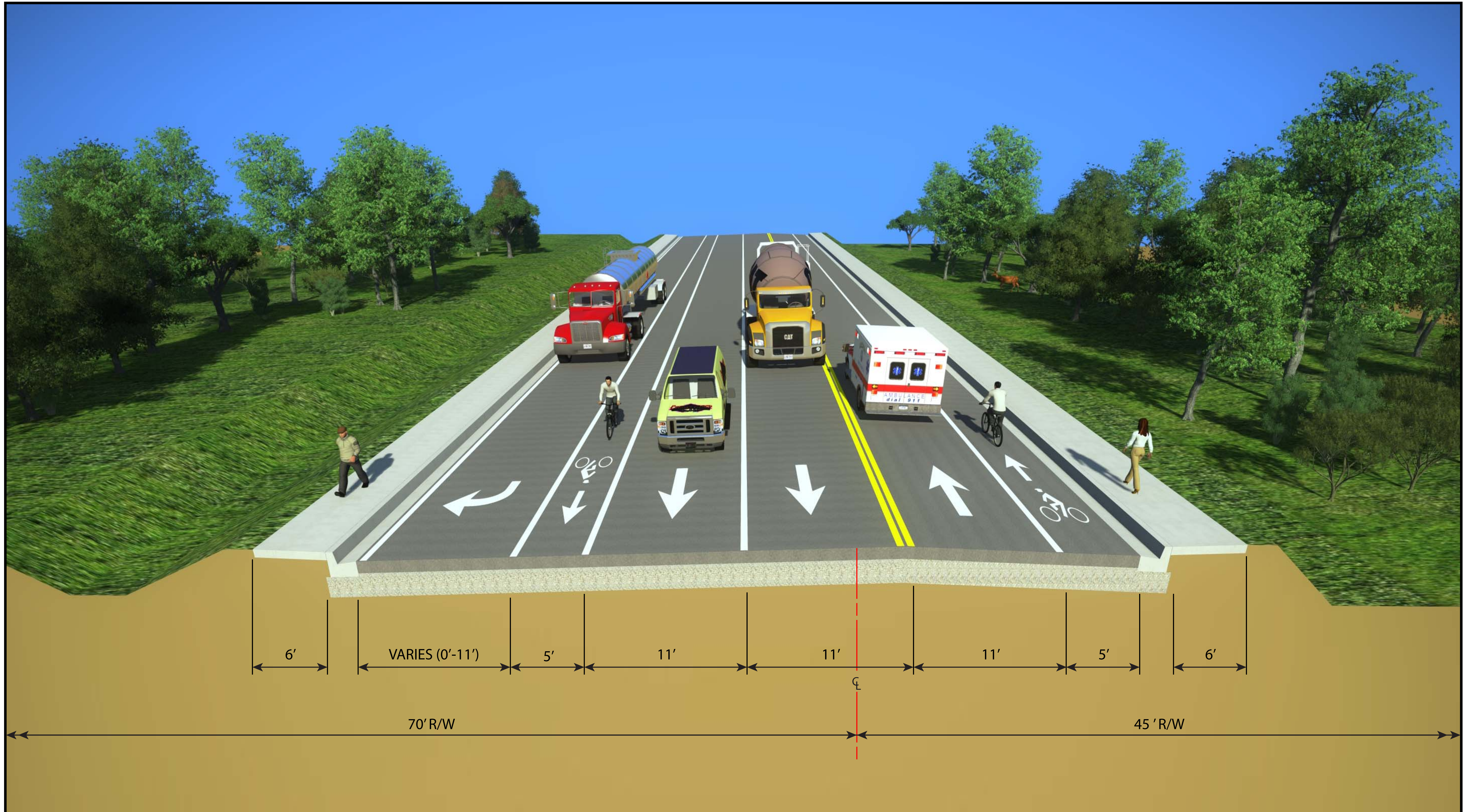
Typical Section - Segment 5 - Tram Road
