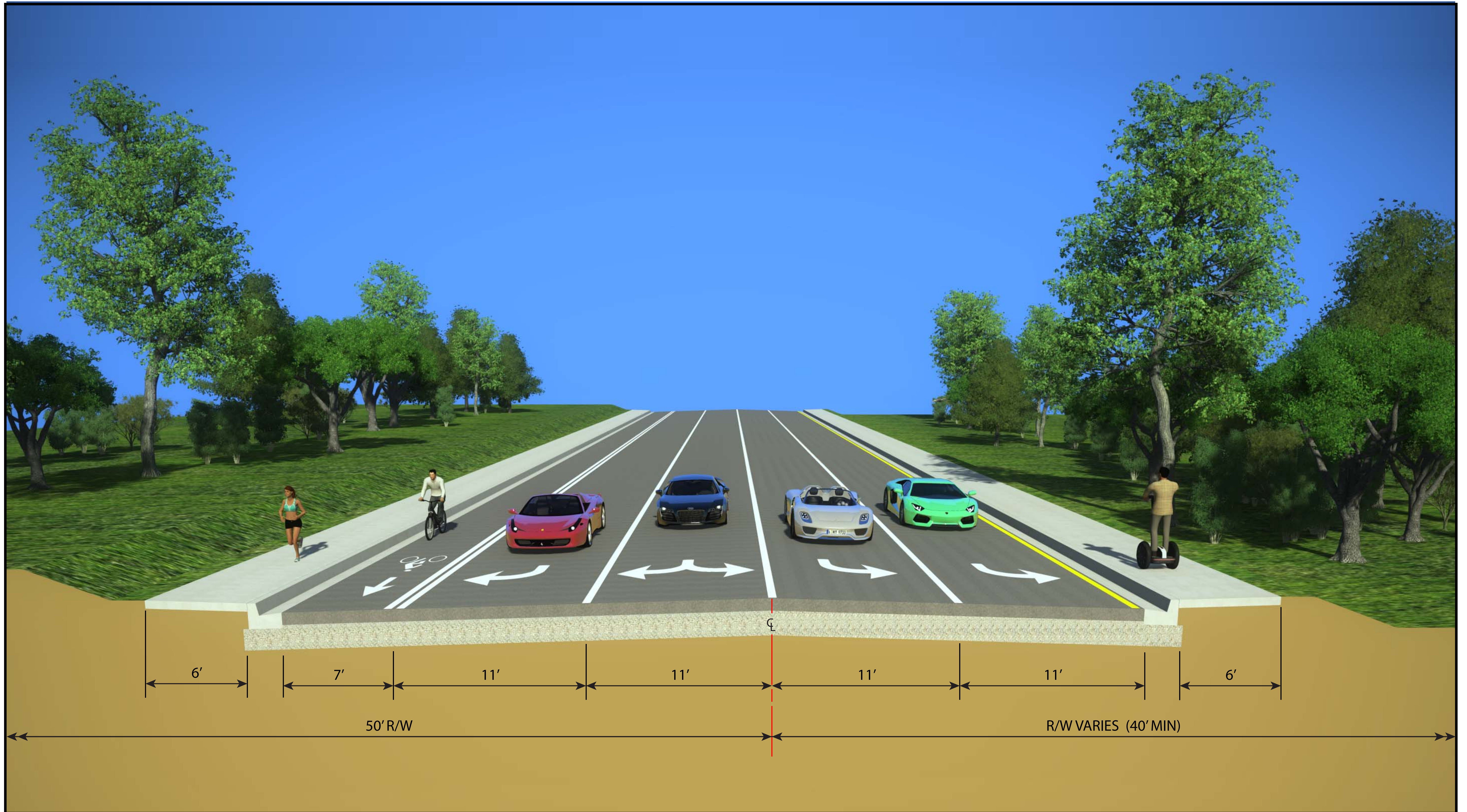
Typical Section - Segment 5 - Tram Road Extension
