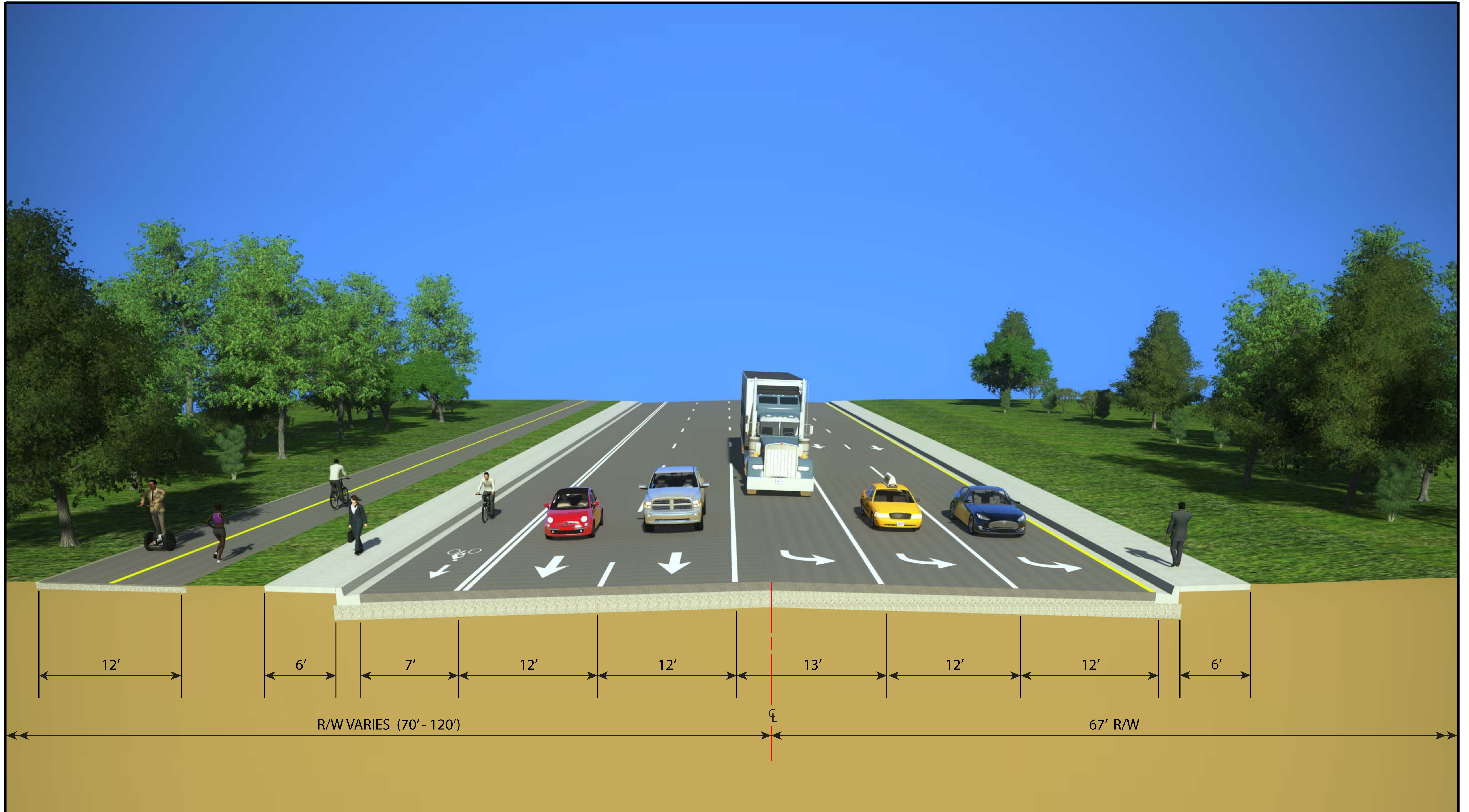
Typical Section - Segment 5 - S.R. 61 (Crawfordville Road)
