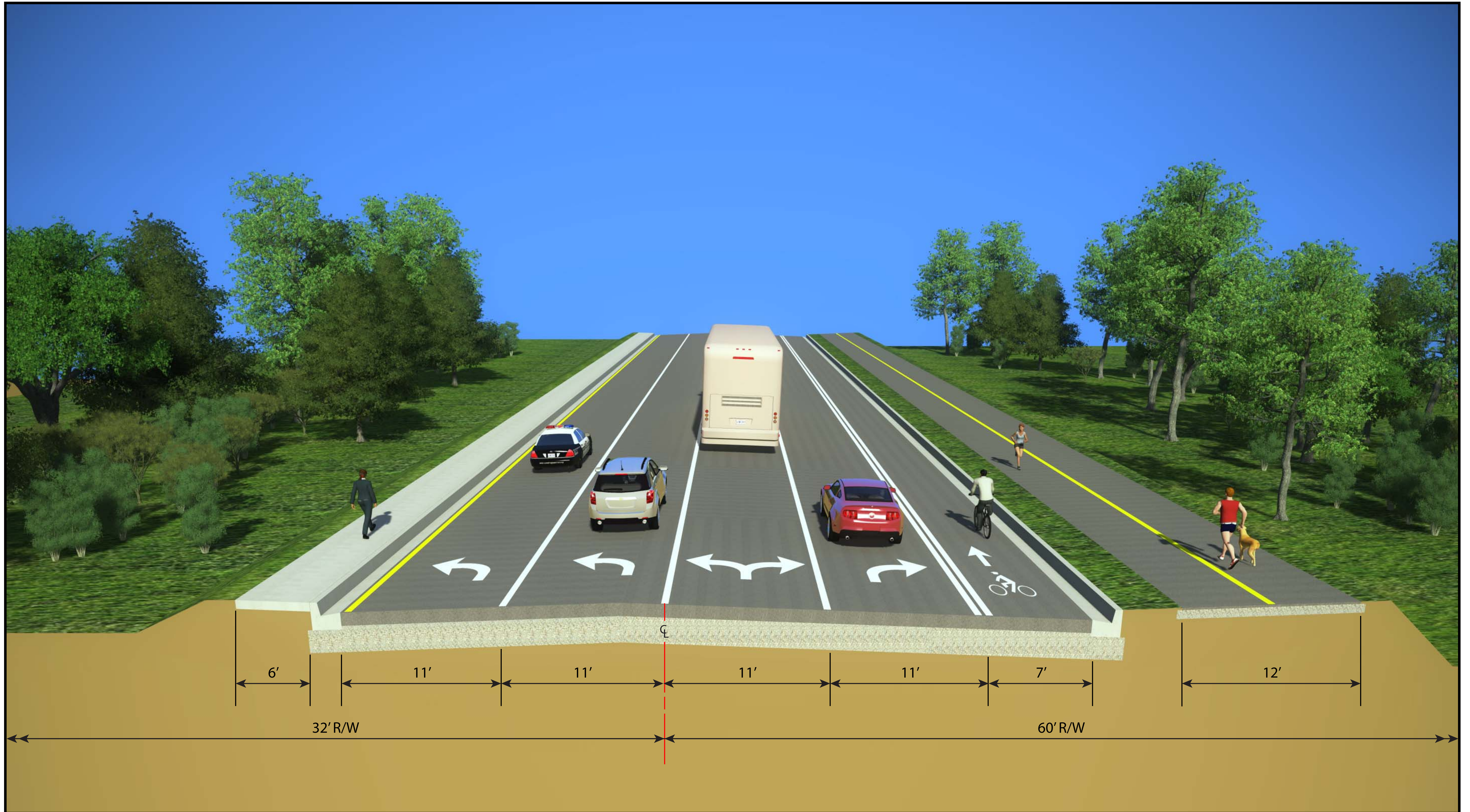
Typical Section - Segment 5 - Gaile Avenue
