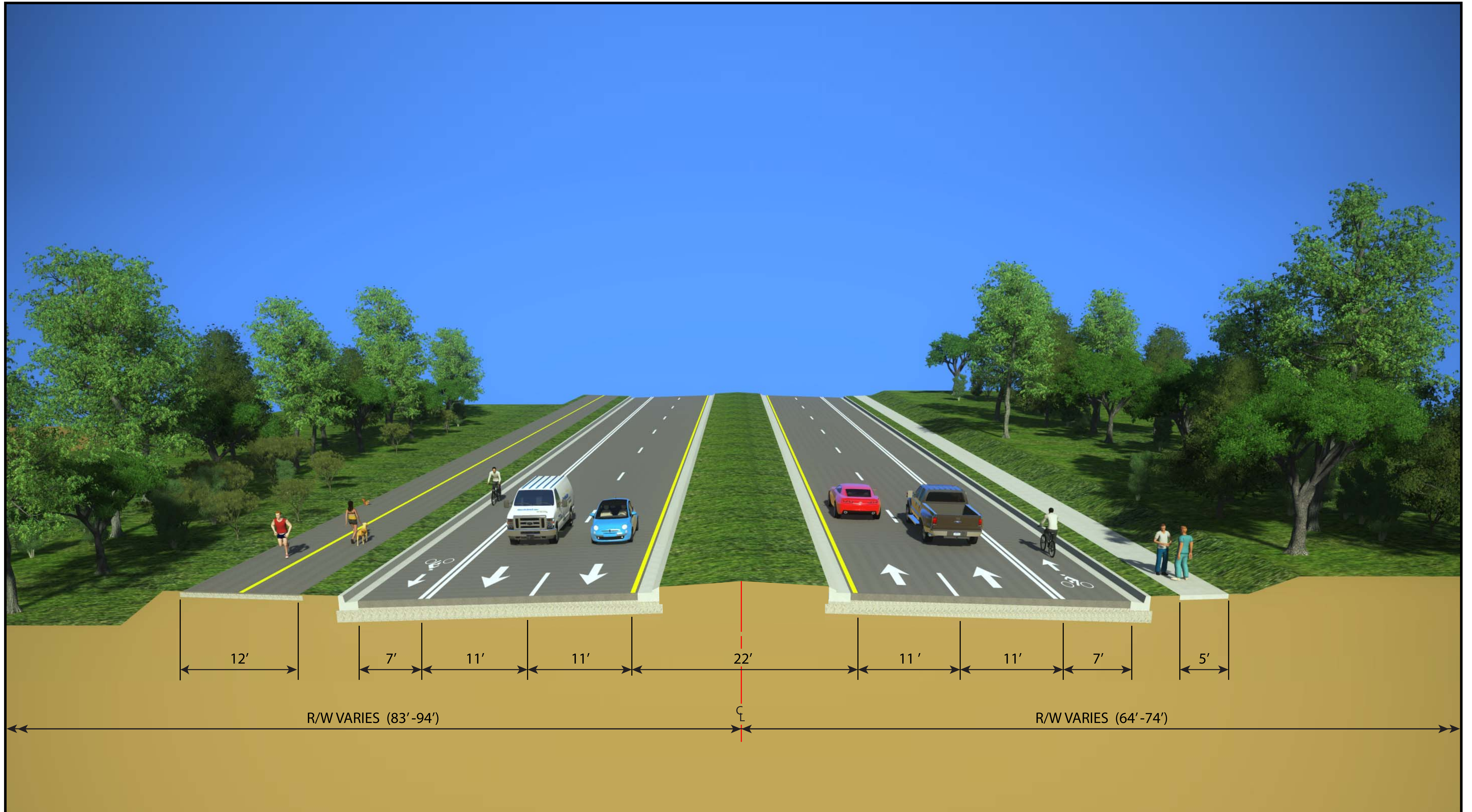
Typical Section - Segment 4 - S.R. 363 (Woodville Highway)
