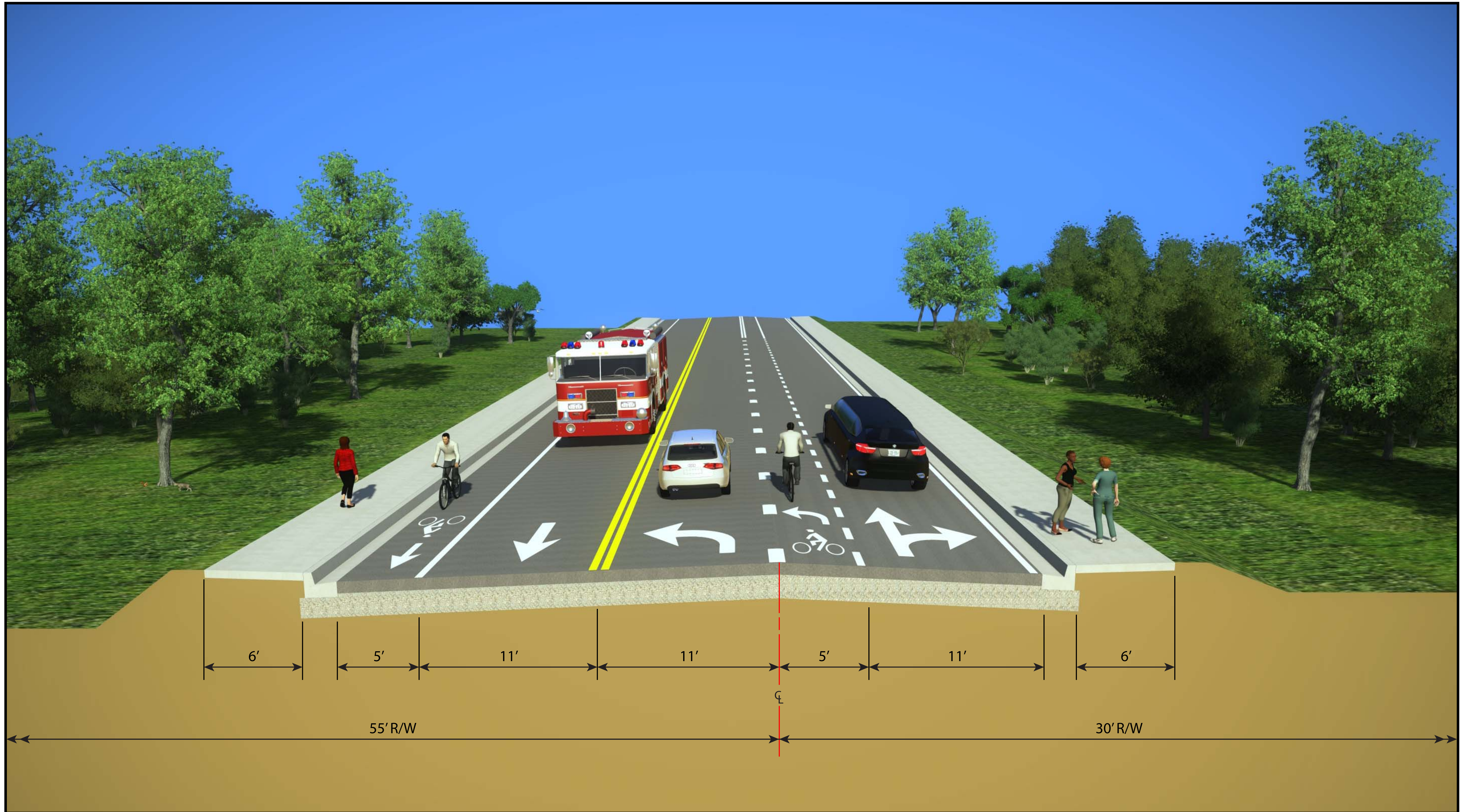
Typical Section - Segment 4 - Ross Road
