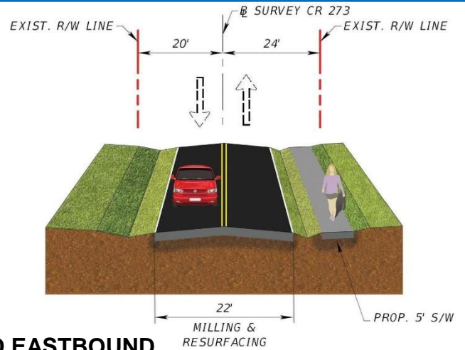
SOUTH BOULEVARD EASTBOUND
