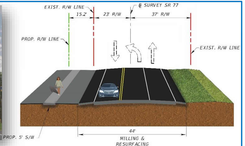
STATE ROAD 77 (MAIN STREET) NORTHBOUND
