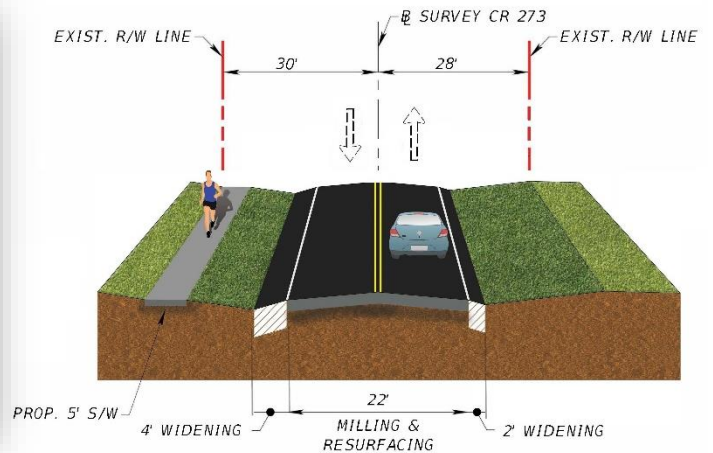
SOUTH BOULEVARD WESTBOUND
